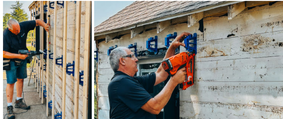
Installing using nails
